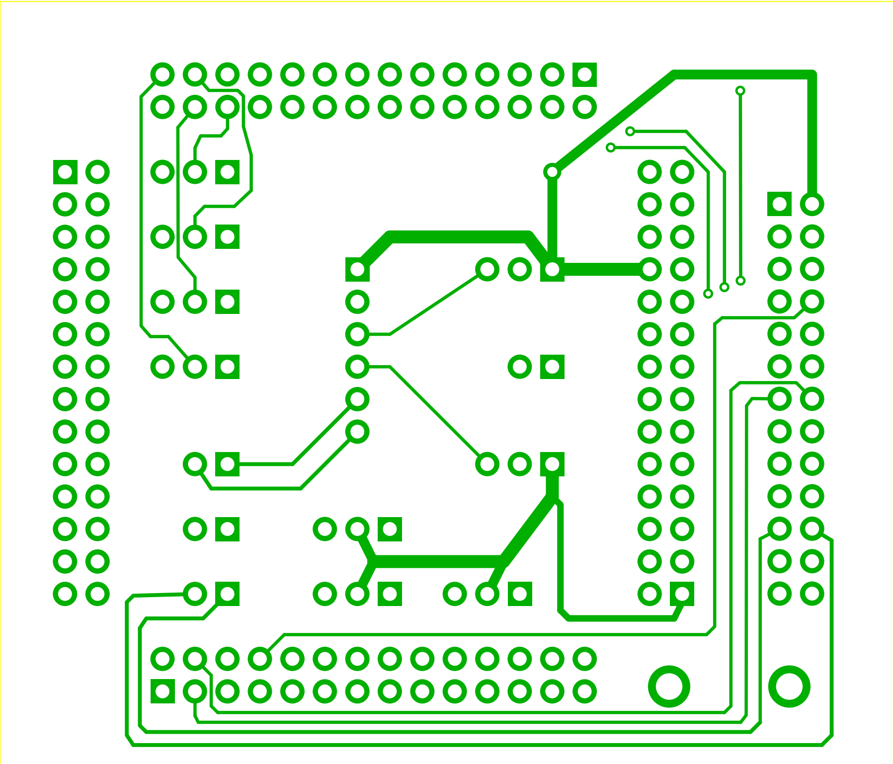
MiniDragonDOTRBRD_12Vmod_RevF_JCH.pcb (Bottom layer)
