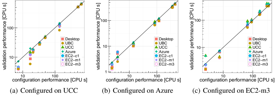
Fig. 1. Validation performance ( \log_{10} runtime) for Spear configurations found in 8 ParamILS runs with different random seeds on 3 different infrastructures. The shapes/colours denote the infrastructure the configuration was validated on.
