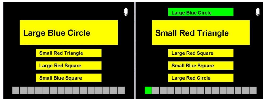
Figure 1. Display for multimodal configurations using an abstracted task list. The display is rendered on one of three hardware configurations and is paired with audio, touch, and/or speech recognition.
