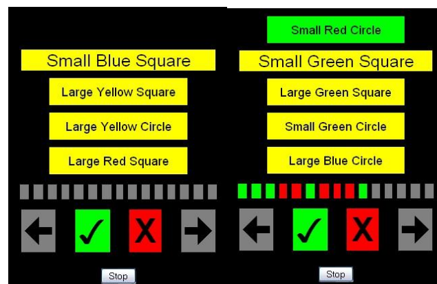
Figure 2. Visual display for handheld configuration using an abstracted task list. Left: the handheld GUI when the application starts. Right: the GUI after several items have been checked off. The most recently checked item is green because it passed inspection, and the progress bar is color coded according to the inspection results of all items checked so far.
