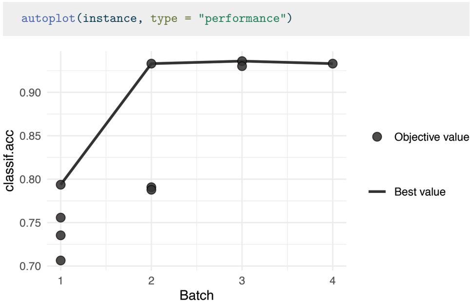
Figure 6.2: Model performance in iterations of sequential forward selection.
