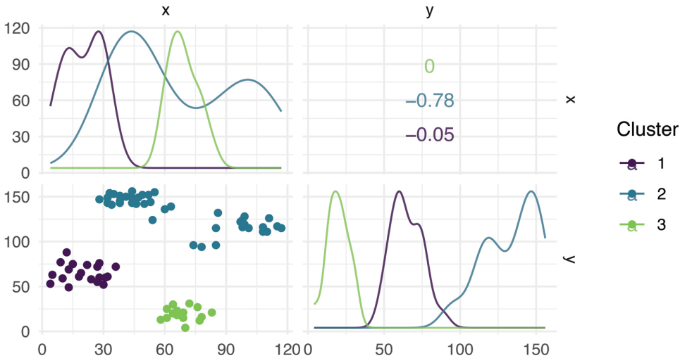
Figure 13.7: Distribution of the estimated clusters.
