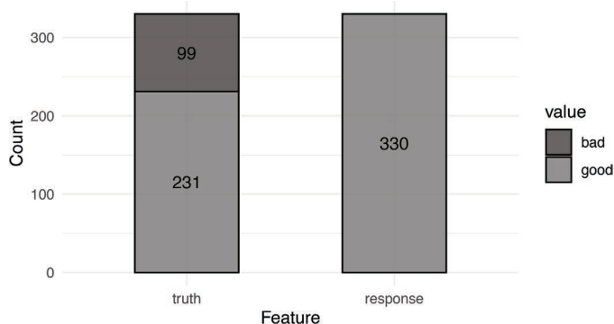
Figure 2.6: Class labels ground truth (left) and predictions (right). The learner completely ignores the “bad” class.
