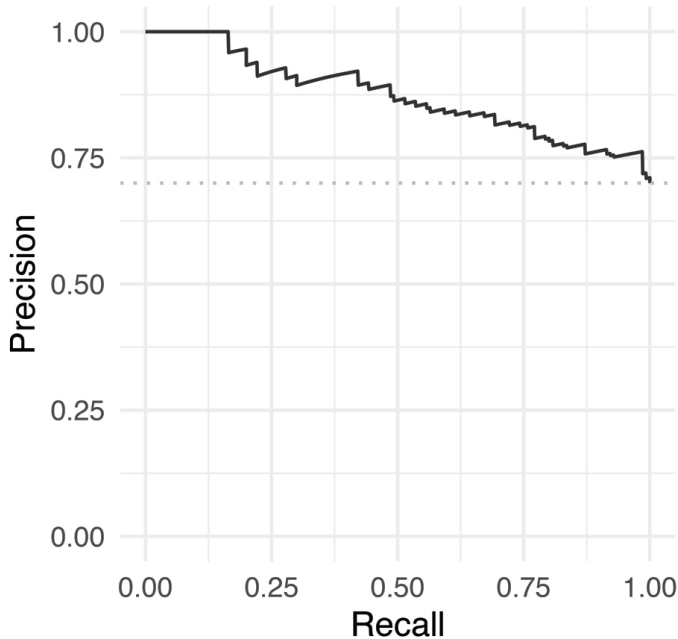
Figure 3.12: Precision-Recall curve based on tsk("german_credit") and lrn("classif.ranger") .
