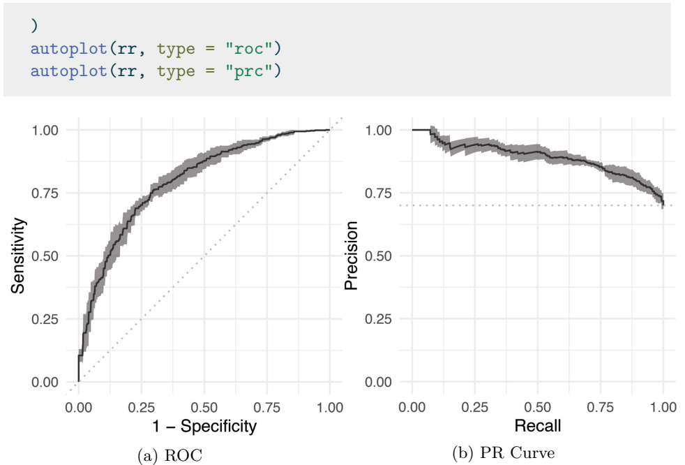
Figure 3.14: Comparing ROC (left) and PR curve (right) for a random forest trained on tsk("german_credit") .
