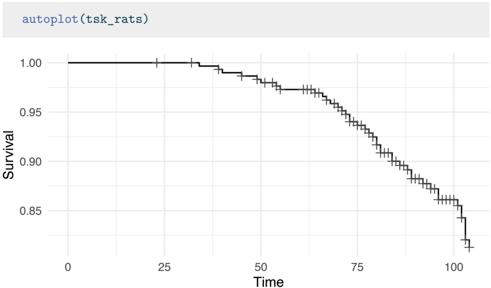
Figure 13.3: Kaplan-Meier plot of tsk("rats") . x-axis is time variable and y-axis is survival function, S(T) , defined by 1 - F(T) where F is the cumulative distribution function. Crosses indicate points where censoring takes place.
