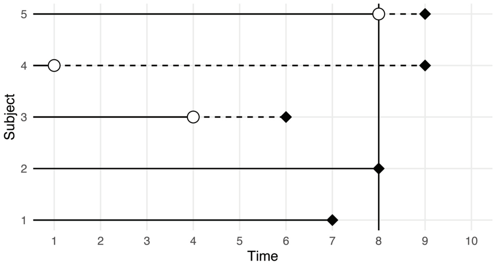
Figure 13.2: Plot illustrating different censoring types. Dead and censored subjects (y-axis) over time (x-axis). Black diamonds indicate true death times and white circles indicate censoring times. Vertical line is the study end time. Subjects 1 and 2 die in the study time. Subject 3 is censored in the study and (unknown) dies within the study time. Subject 4 is censored in the study and (unknown) dies after the study. Subject 5 dies after the end of the study. Figure and caption from R. E. B. Sonabend (2021).
